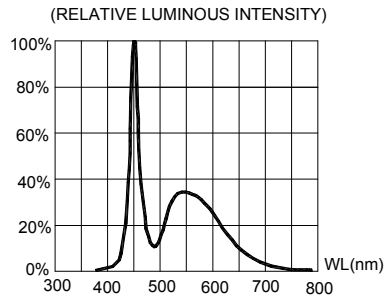
FIG.4 RELATIVE LUMINOUS INTENSITY VS. WAVELENGTH. 50% Power Angle : 105°
