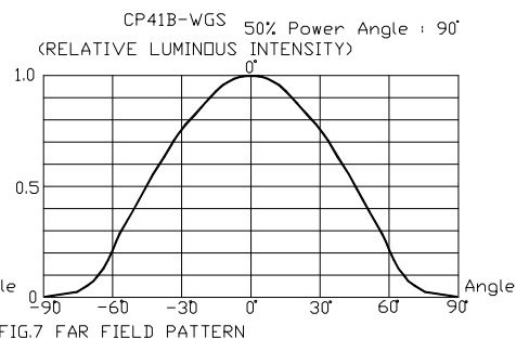
FIG.7 FAR FIELD PATTERN
