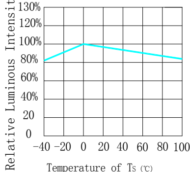
Fig.4 Relative Intensity Vs Temperature of T_s
