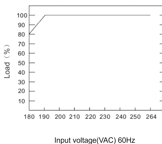
■ Input Derating Curve
