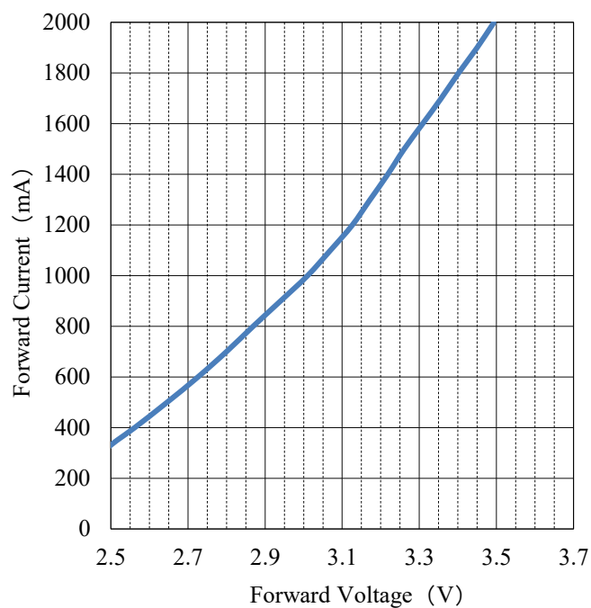
Forward Voltage VS Forward Current T_s=85^\circ\text{C}
