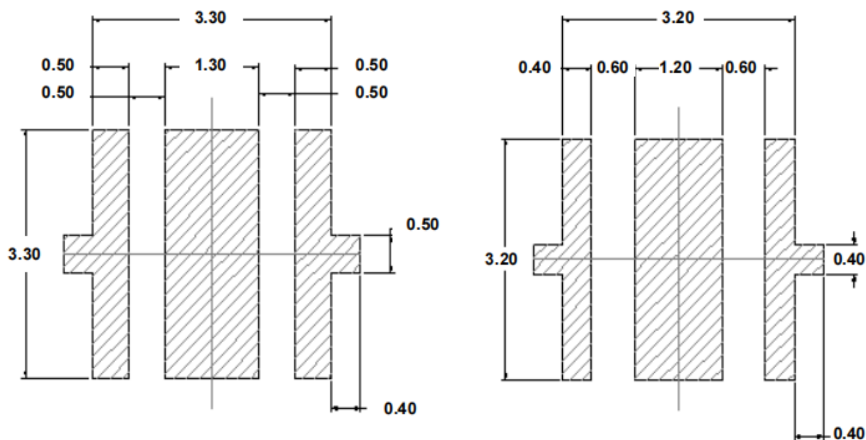
Recommended PCB Solder Pad
