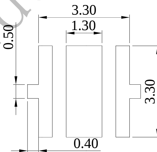
Soldering Patterns
