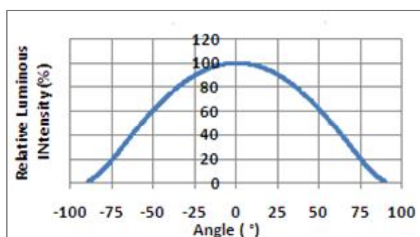
Fig.6-Radiation diagram
