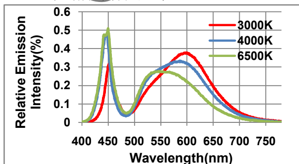
Fig.7- Spectrum Distribution
