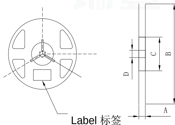
Fig.2-2 Reel Dimension 卷盘尺寸
