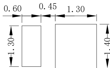
Fig.1-5 Soldering Patterns 推荐焊盘
