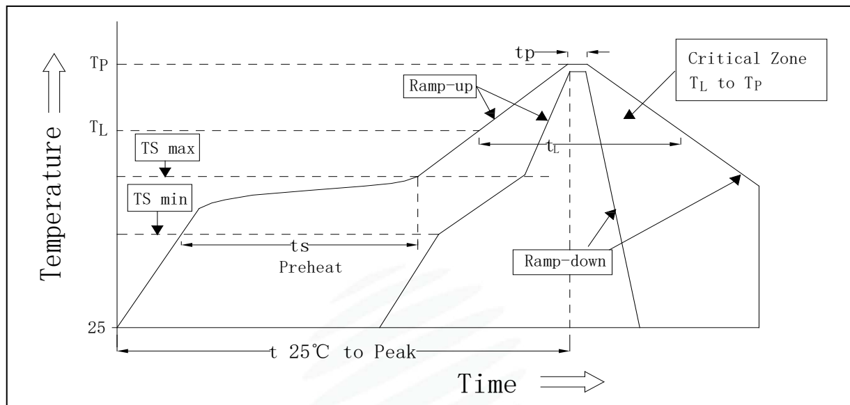
Fig.3-1 SMT Reflow Soldering Instructions SMT 回流焊说明
