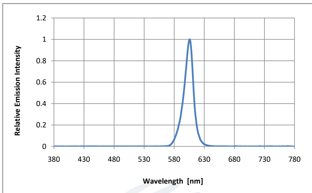
Fig 1-12 Spectrum Distribution光谱分布特性曲线
