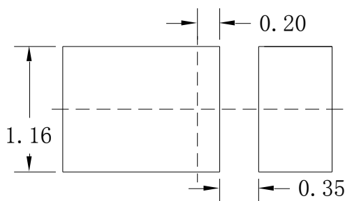
Fig.1-5 Soldering patterns 推荐焊盘
