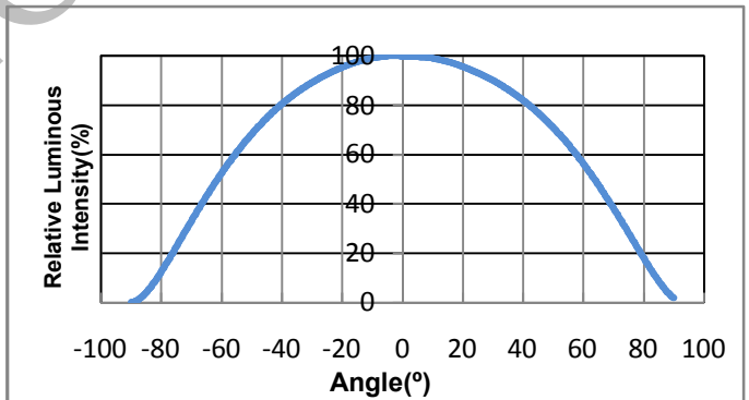
Fig.6- Radiation diagram
