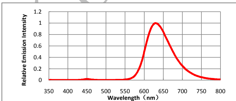
Fig.7- Spectrum Distribution
