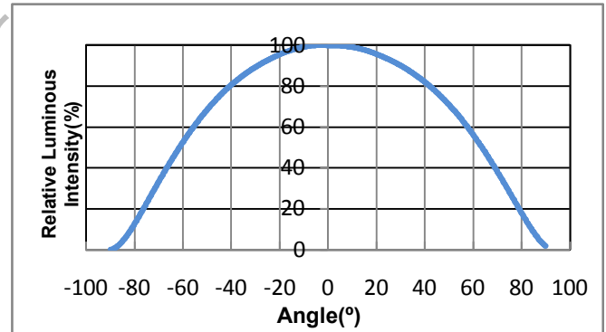
Fig.6- Radiation diagram
