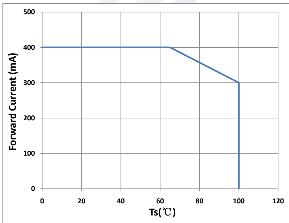
Fig 1-10 Solder Temperature Vs. Forward Current 管脚温度与正向电流特性曲线 (Ts=25°C)
