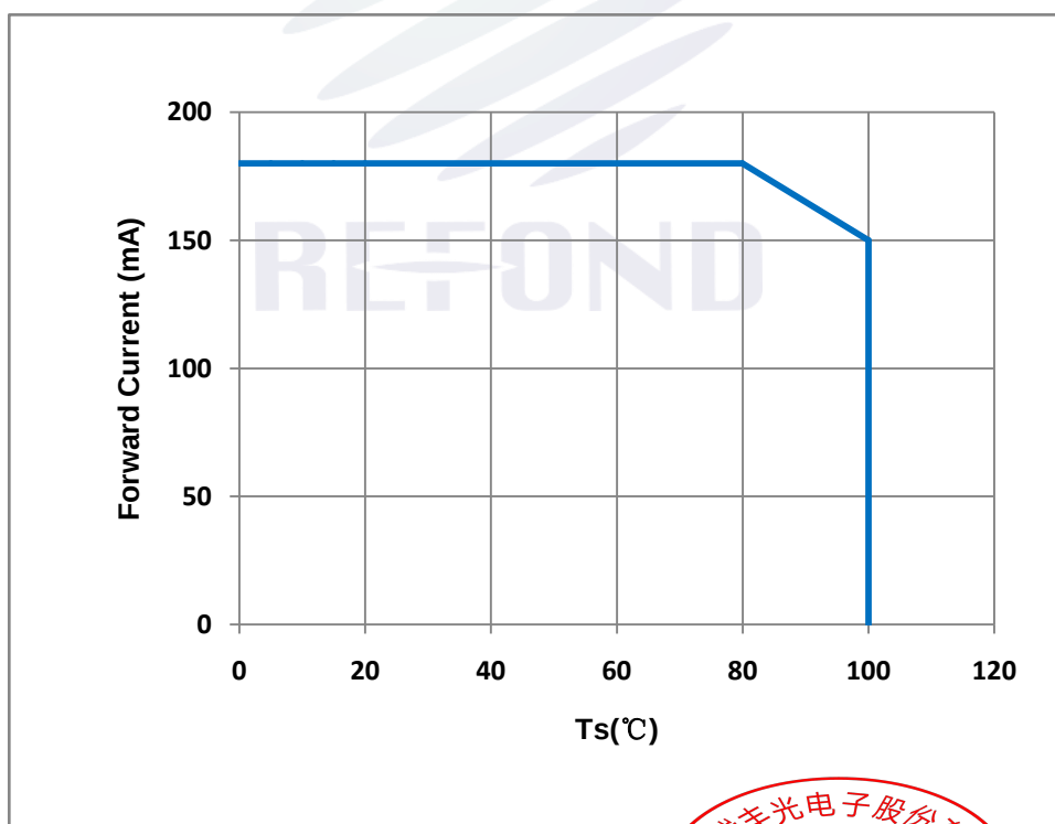
Fig 1-12 Solder Temperature Vs. Forward Current 管脚温度与正向电流特性曲线
