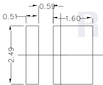
Fig.1-5 Soldering patterns 推荐焊盘
