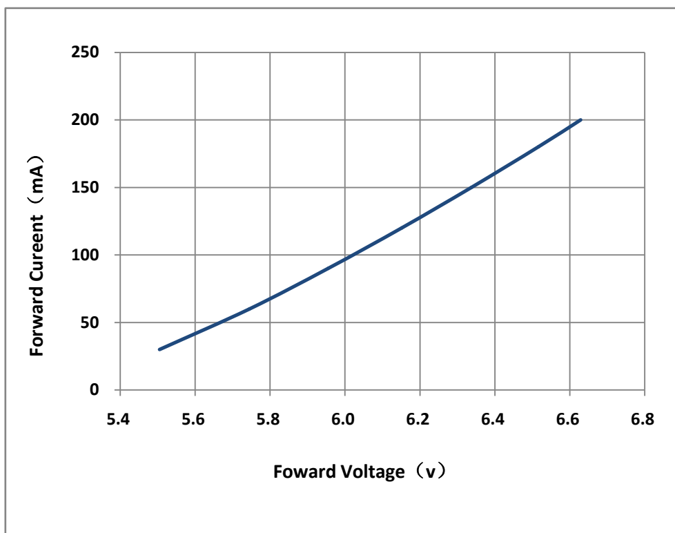
Fig 1-9 Forward Voltage Vs. Forward Current 伏安特性曲线
