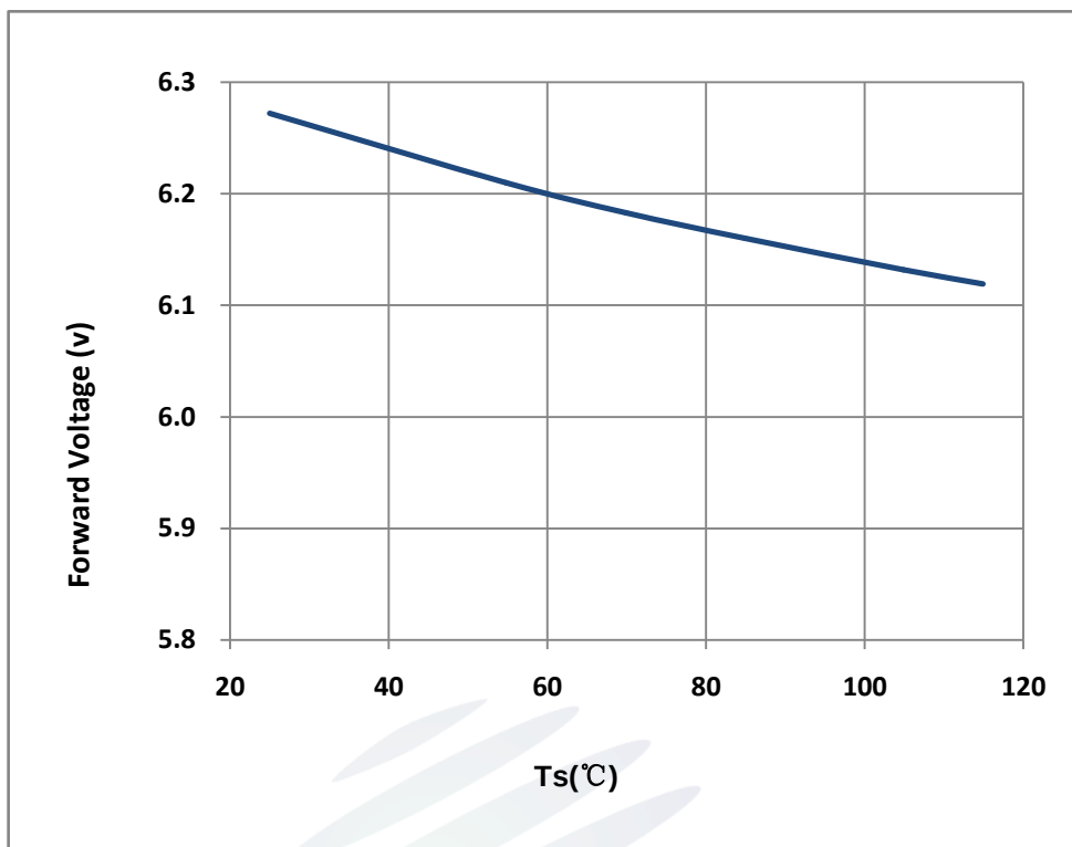
Fig 1-13 Forward Voltage Vs Solder Temperature 电压与管脚温度特性曲线
