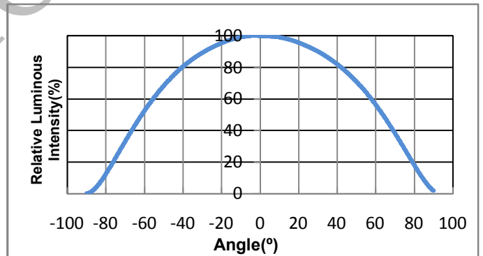
Fig.6-Radiation diagram
