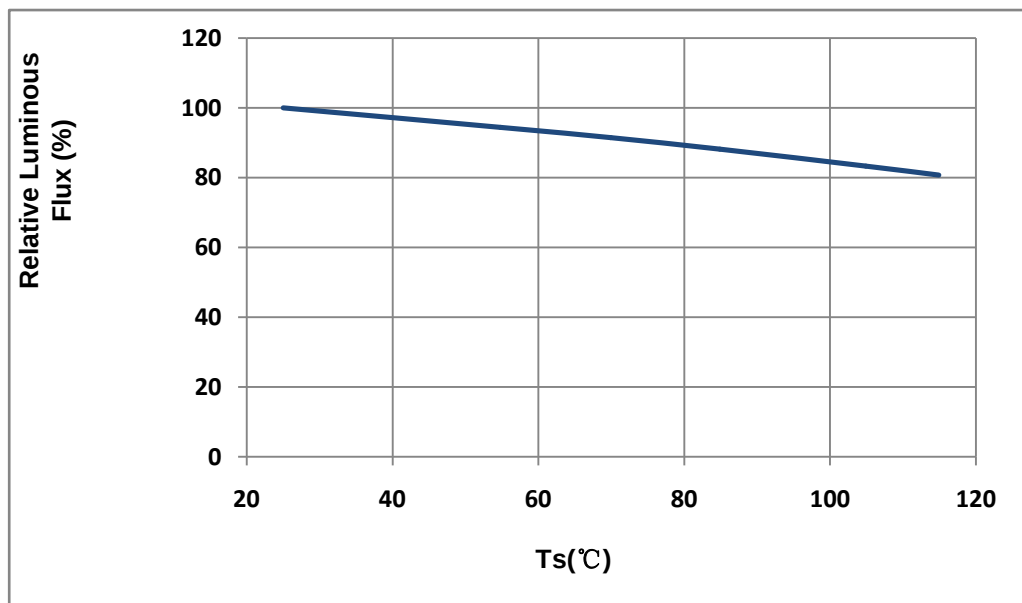
Fig 1-11 Solder Temperature Vs Relative Intensity 管脚温度与相对光强特性曲线
