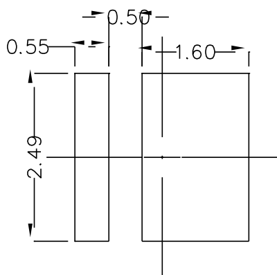
Fig.1-5 Soldering patterns
