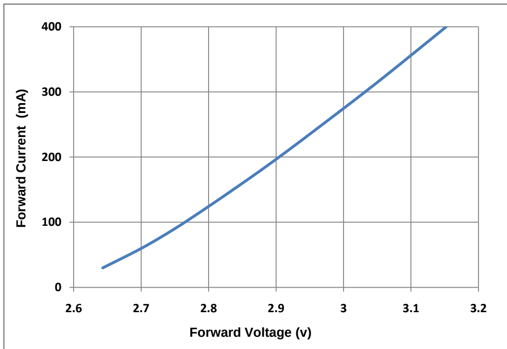
Fig 1-7 Forward Voltage Vs. Forward Current 伏安特性曲线 T_s=25^{\circ}\text{C}
