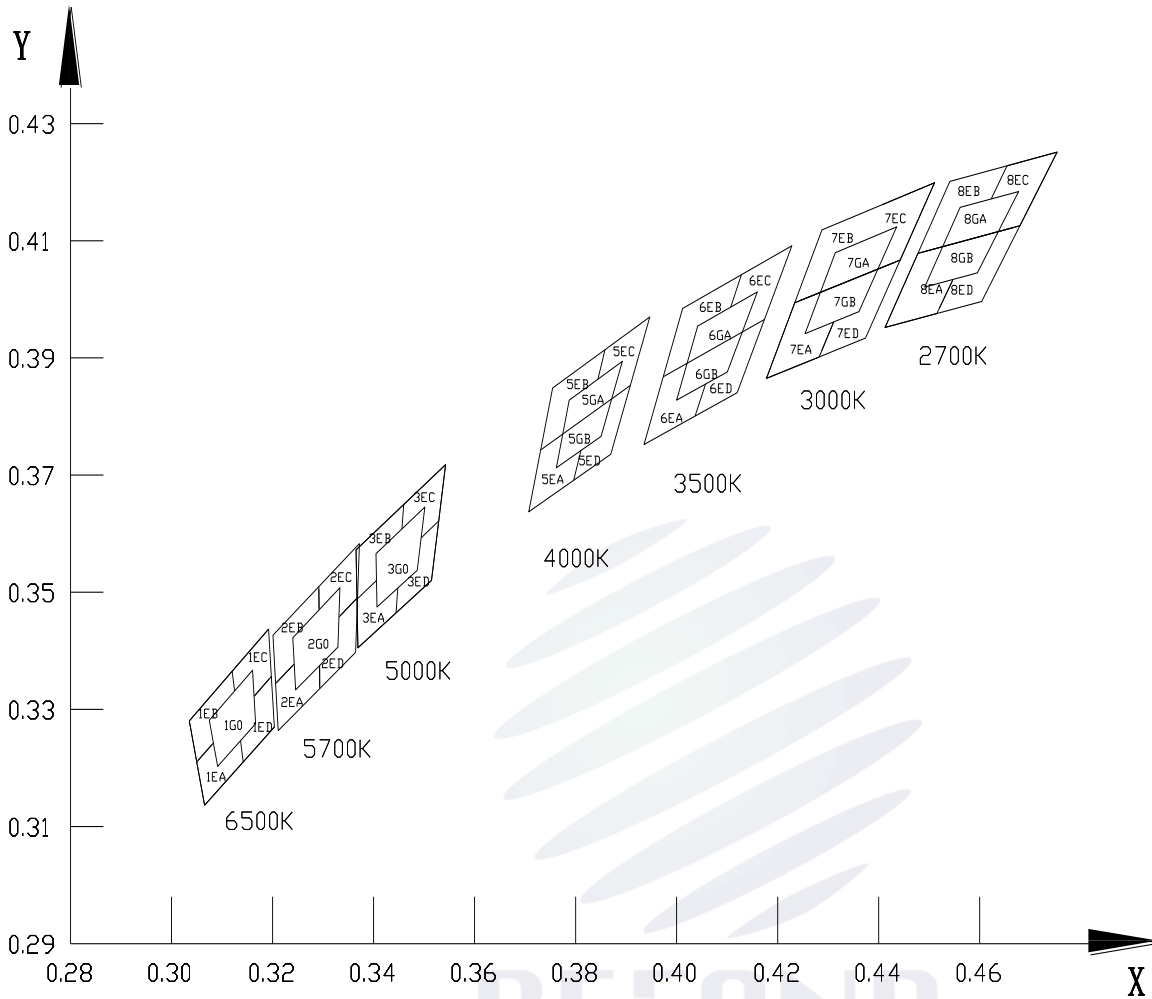
Fig 1-6 The C.I.E Chromaticity Diagram CIE色度图
