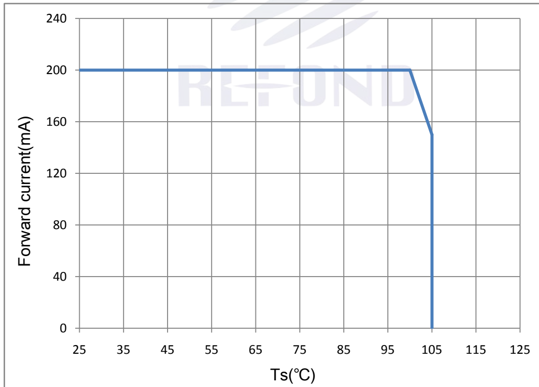
Fig. 1-10 Solder Temperature Vs Forward Current 管脚温度与正向电流特性曲线 T_j \leq 125^\circ\text{C}
