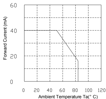
Derating
