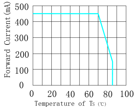
Fig.3 Forward Current Vs Temperature of T_s
