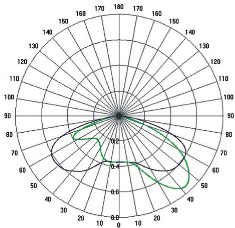
Light distribution curve
