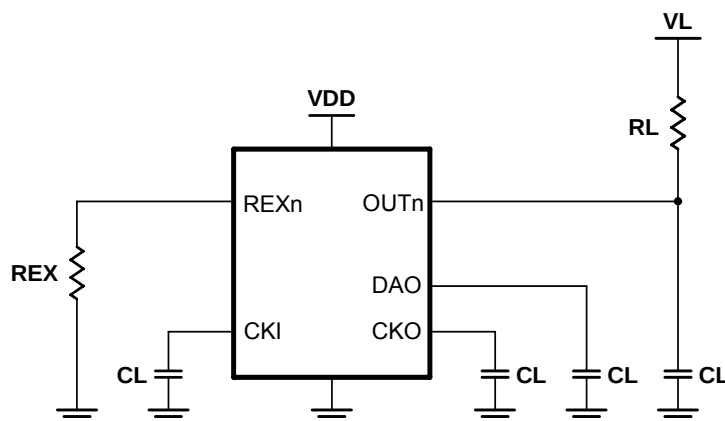
Switching Characteristics Test Circuit
