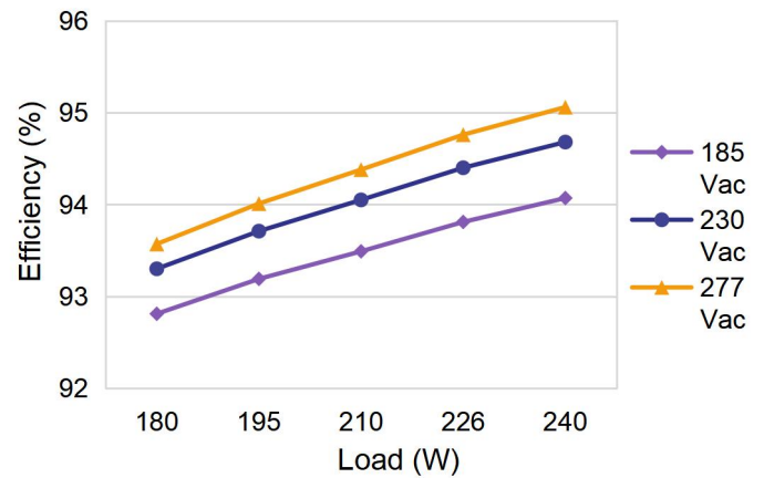
Typical Efficiency vs Load
