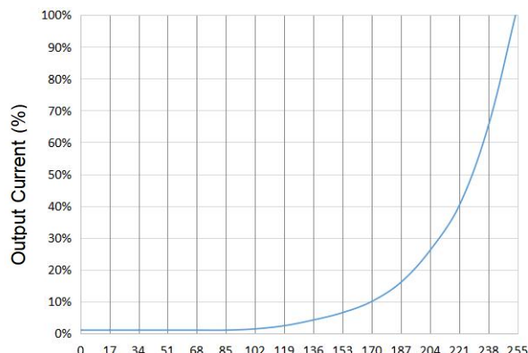
Logarithmic dimming
