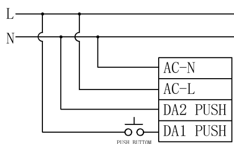
Wiring diagram of PUSH dimming
