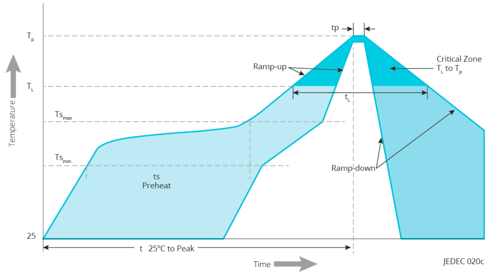
Figure 14. Visualization of the acceptable reflow temperature profile as specified in Table 12.
