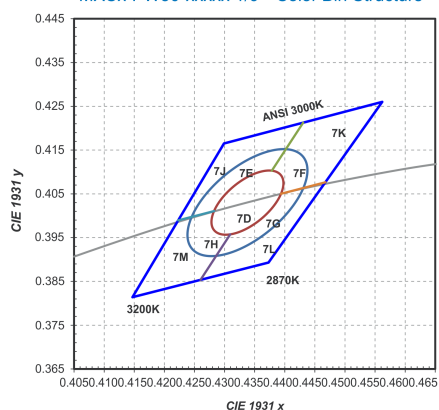
MXCx-PW30-xxxxx 1/6 th Color Bin Structure
