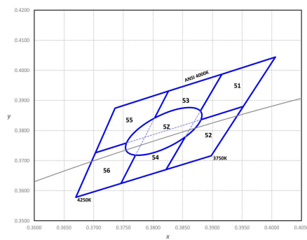
Color bin structure for LUXEON 3535L Line 4000K.
