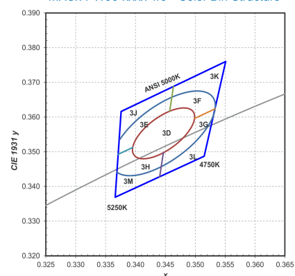
MXCx-PW50-xxxx 1/6 th Color Bin Structure
