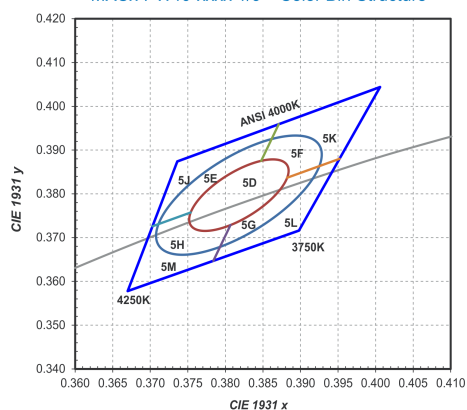
MXCx-PW40-xxxx 1/6 th Color Bin Structure
