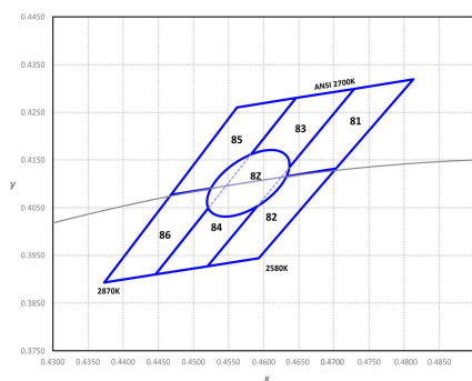
Color bin structure for LUXEON 3535L Line 2700K.
