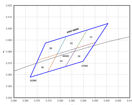
MXCx-PW40-xxxx 1/6 th Color Bin Structure
