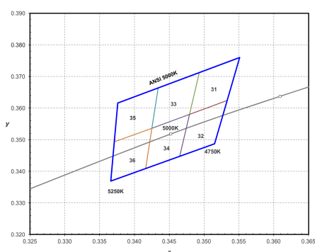
MXCx-PW50-xxxx 1/6 th Color Bin Structure
