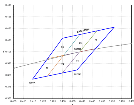
MXCx-PW30-xxxxx 1/6 th Color Bin Structure
