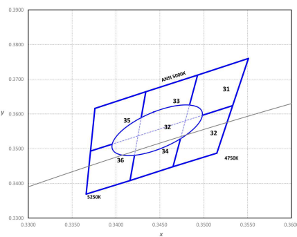
Color bin structure for LUXEON 3535L Line 5000K.
