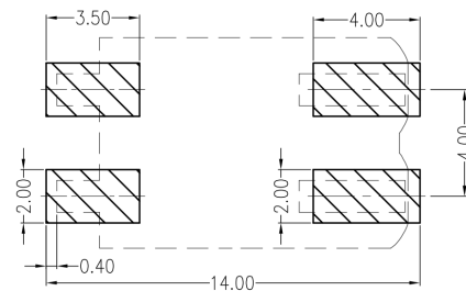
Board Layout
