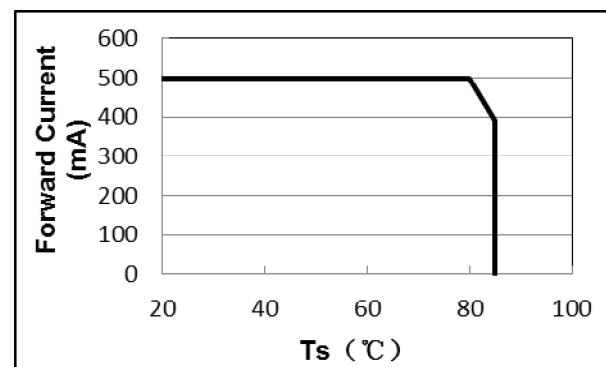
Fig.6-Ts Temperature Vs. Forward Current 焊盘温度与正向电流特性曲线
