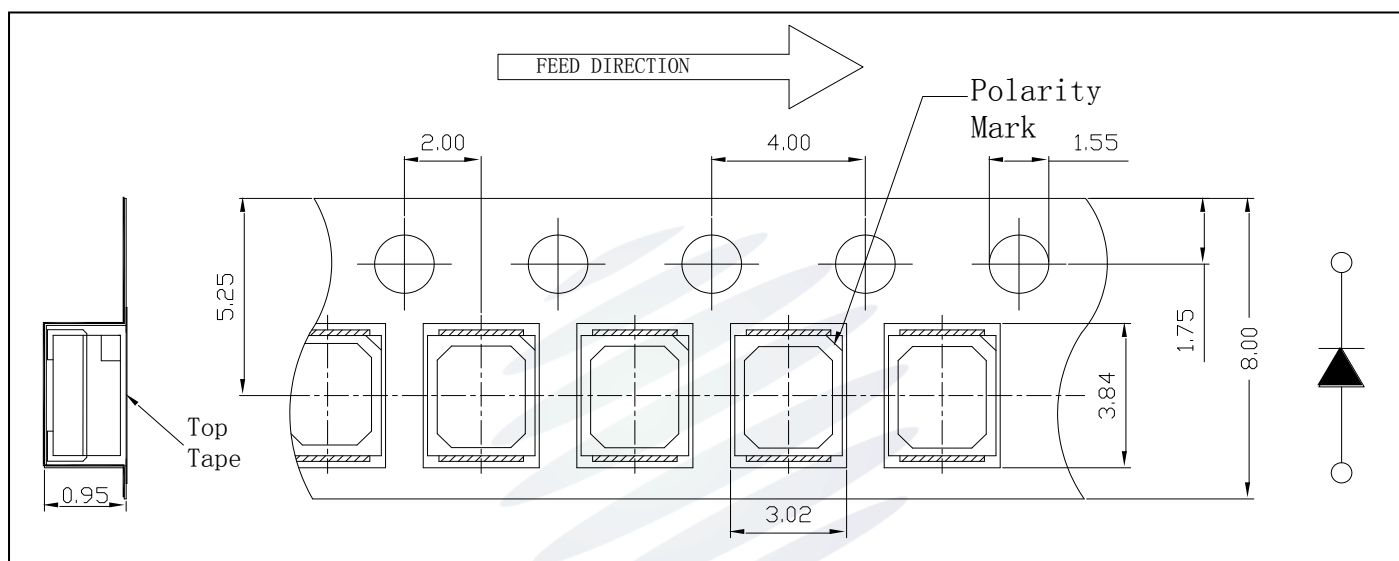
Fig.2-1 Carrier Tape Dimension 載帶尺寸
