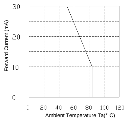
Derating
