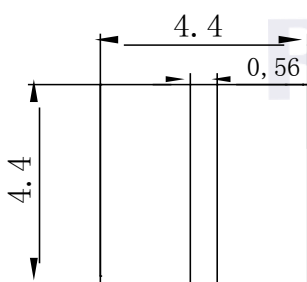
Fig.1-5 Soldering patterns
