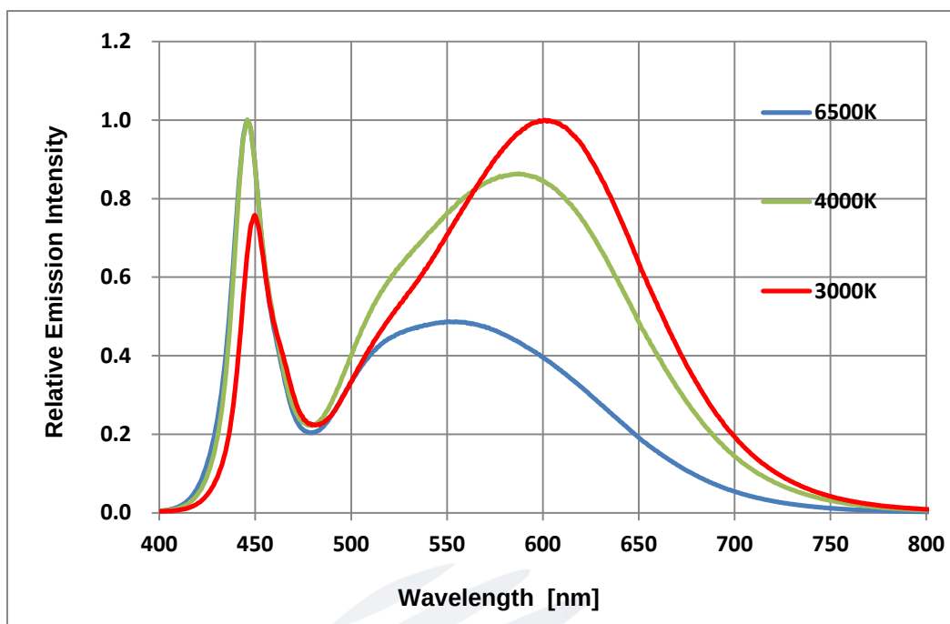
Fig 1-13 Spectrum Distribution
