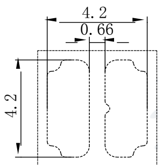
Fig.1-3 Bottom view
