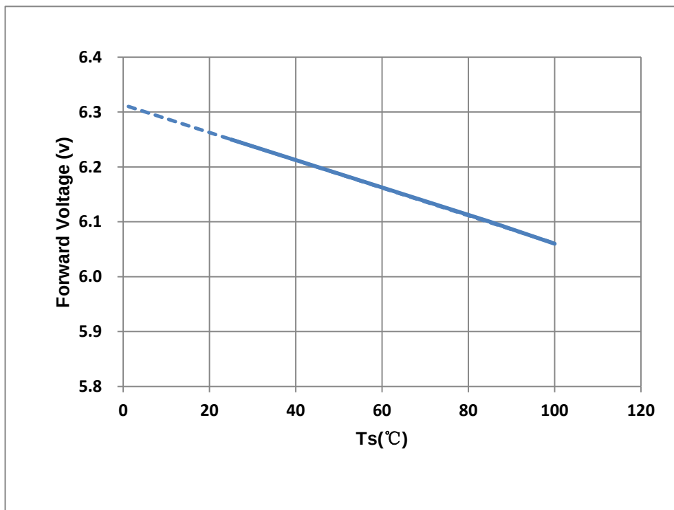
Fig 1-11 Forward Voltage Vs Solder Temperature
