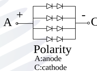
Fig.1-4 Polarity
