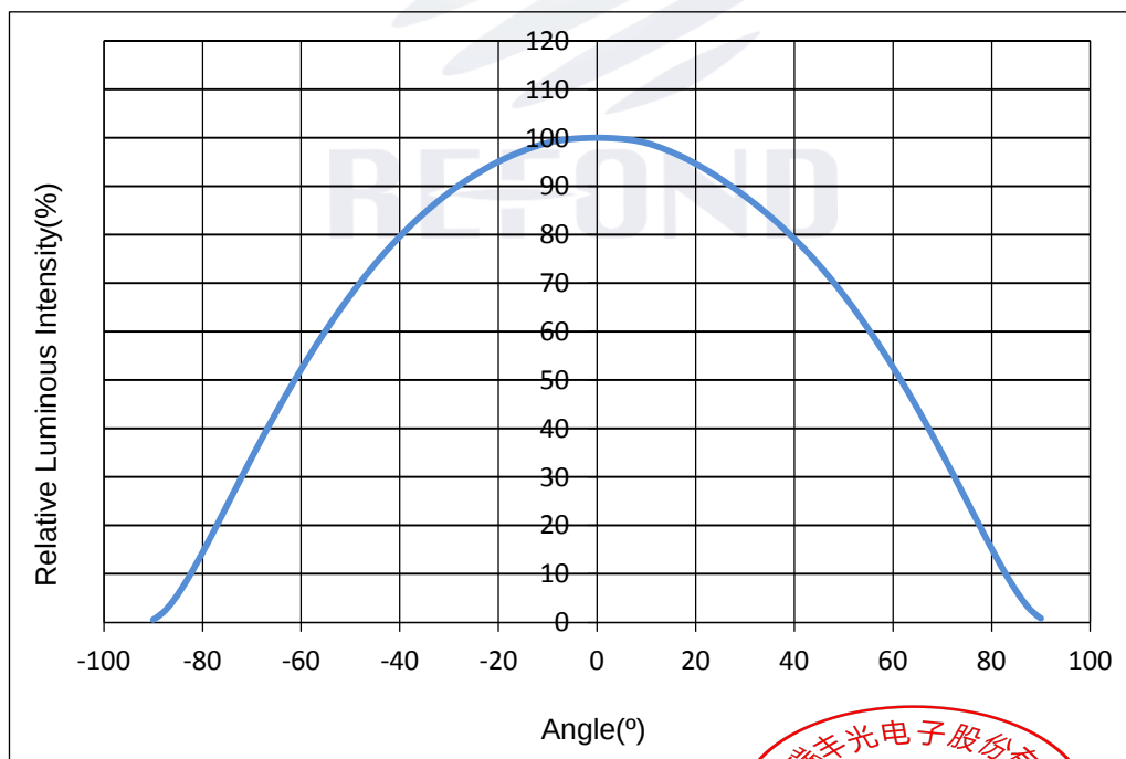
Fig 1-12 Radiation diagram
