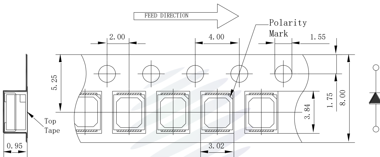
Fig.2-1 Carrier Tape Dimension 載帶尺寸
