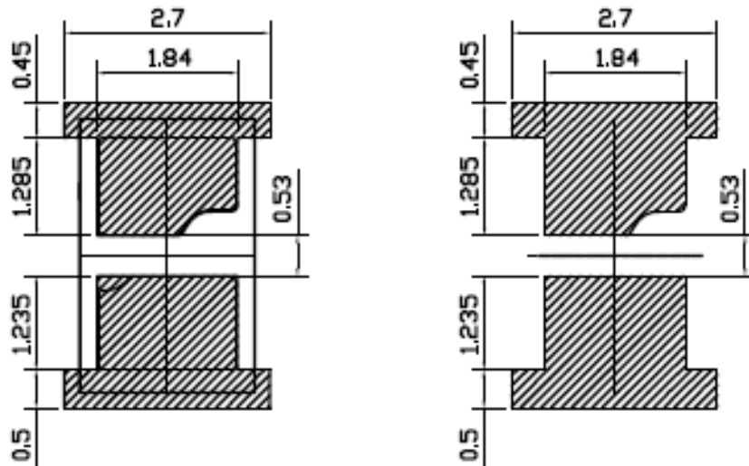
Recommend Land Pattern
