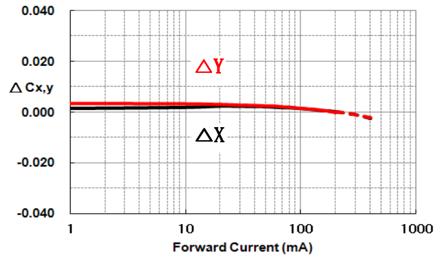
Chromaticity Coordinate Shift
