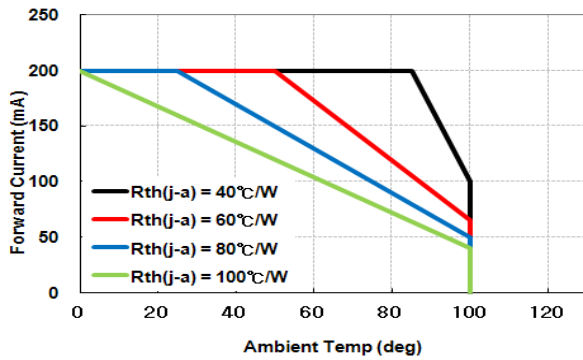
Derating Curve
