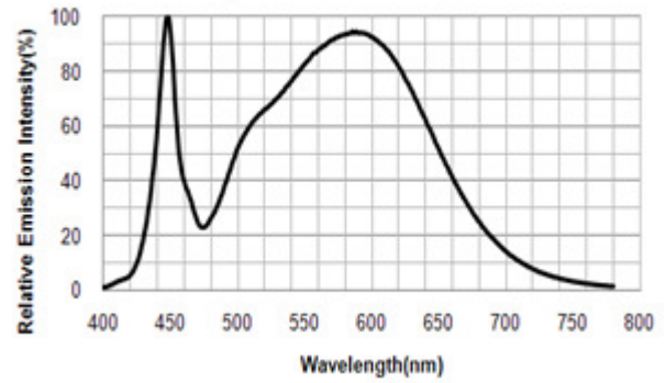
Spectrum Distribution
