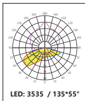
DK-173-135*55-TPIV-S-H-12H1
