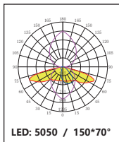
DK-5050-150*70-TPIII-SCL-LENS-6H1
