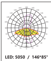
DK-5050-146X85-TP-II-M-FULL-CUTOFF-10H1-NN1
