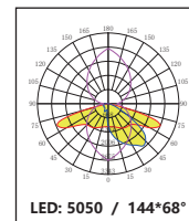
DK-5050-144*68-Semi-Cutoff-TP-III-M-4H1
