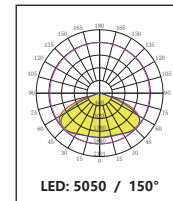
DK-5050-150-TPV-6H1
