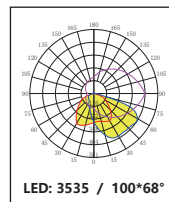
DK-173-100*68-TPIV-S-H-12H1
