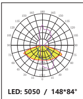
DK-5050-148*84-TPII-M-8H1-Cutoff
