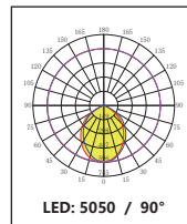
DK-5050-146*83-TP-III-S-8H1-LUMILEDS5050
