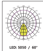
DK-5050-40-8H1-XHWJ-LENS-NN1
