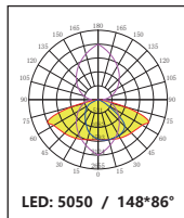
DK-5050-148*86-TPII-M-8H1-Semi-Cutoff
