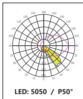
DK-5050-P50-SPORT-6H1
