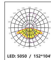
DK-5050-152°104-TPII-M-FULL-CUTOFF-10H1-NN1
