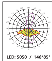
DK-5050-146X85-TPII-M-Cutoff-8H1-B-NN1
